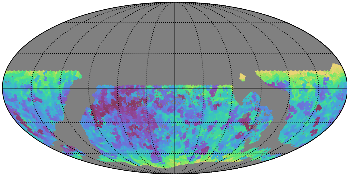
mw_roll_bulge_v3.3_10yrs WFD all bands: Min seeingEff
