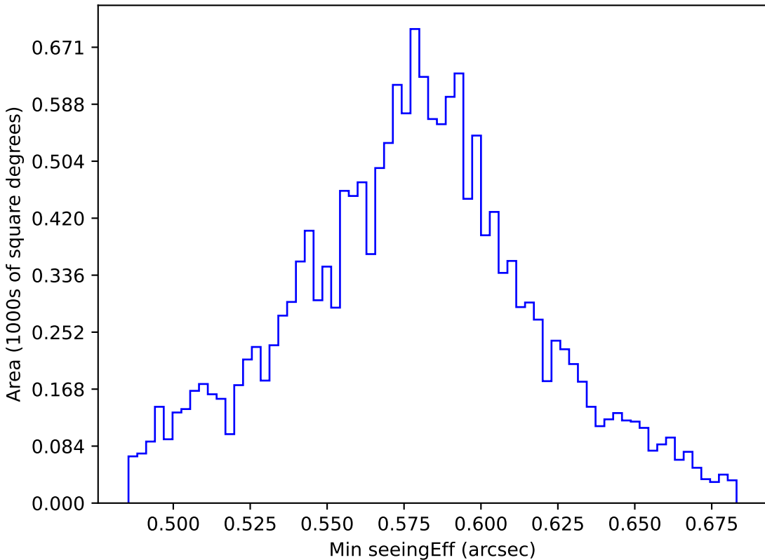
mw_roll_bulge_v3.3_10yrs WFD all bands: Min seeingEff
