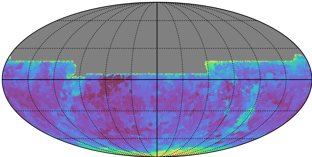
mw_roll_bulge_v3.3_10yrs All sky y band: Min seeingEff
