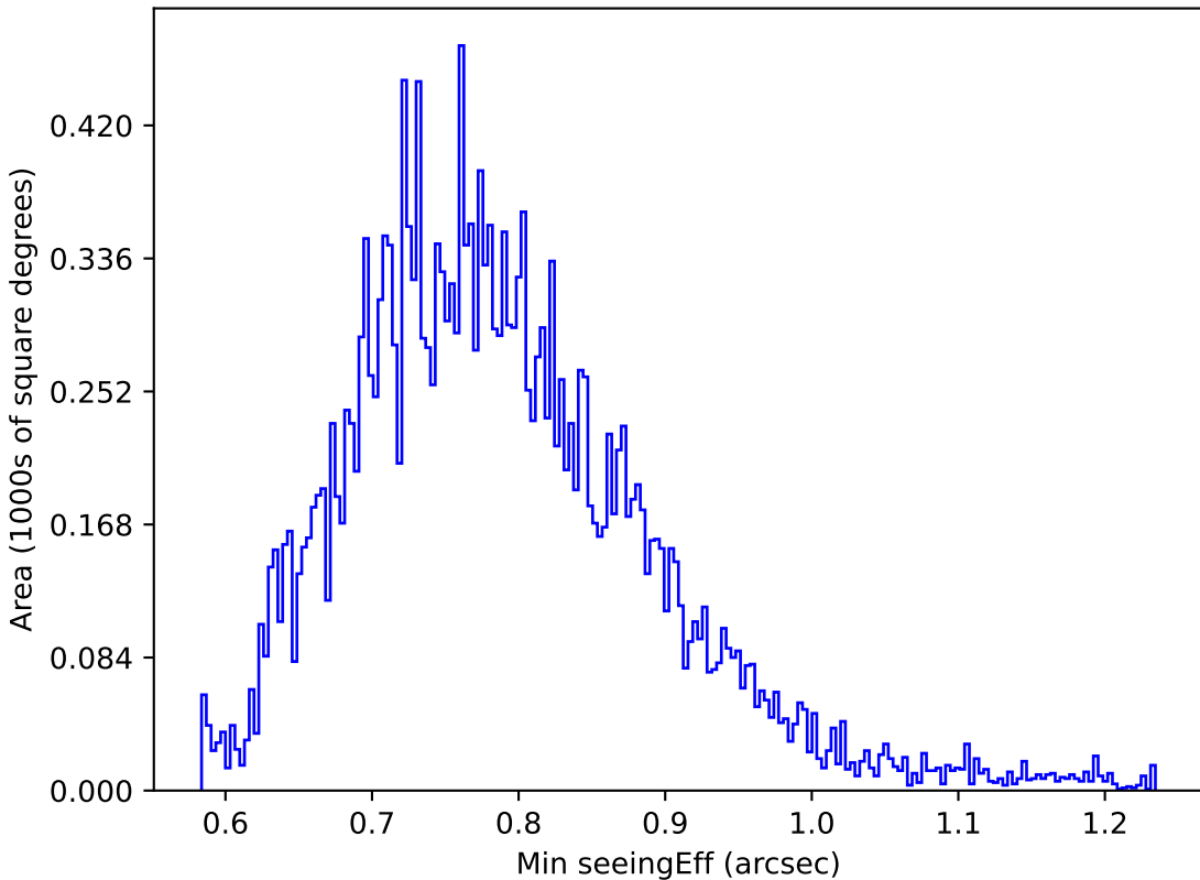
mw_roll_bulge_v3.3_10yrs All sky u band: Min seeingEff
