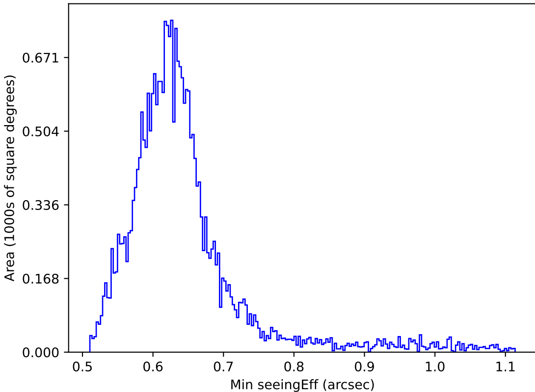
mw_roll_bulge_v3.3_10yrs All sky r band: Min seeingEff
