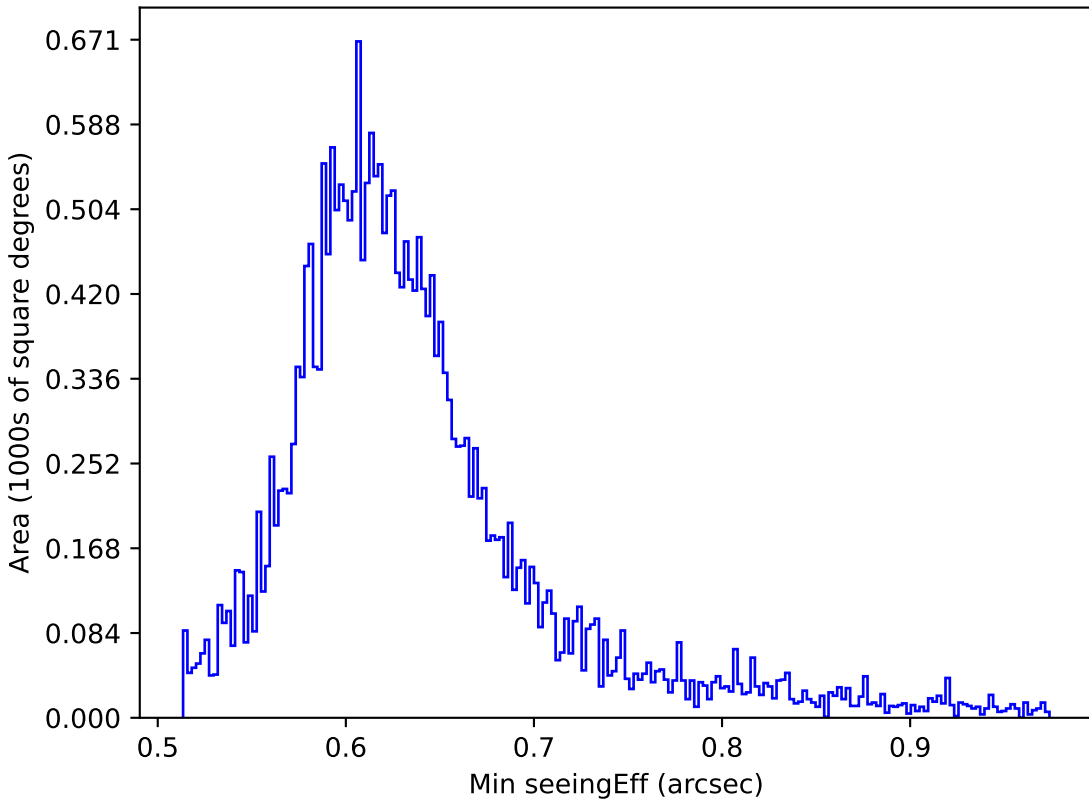
mw_roll_bulge_v3.3_10yrs All sky i band: Min seeingEff
