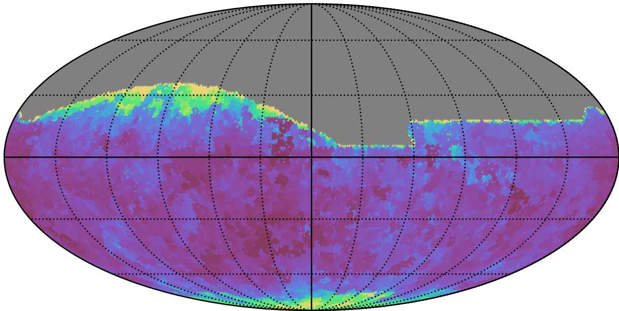
mw_roll_bulge_v3.3_10yrs All sky g band: Min seeingEff
