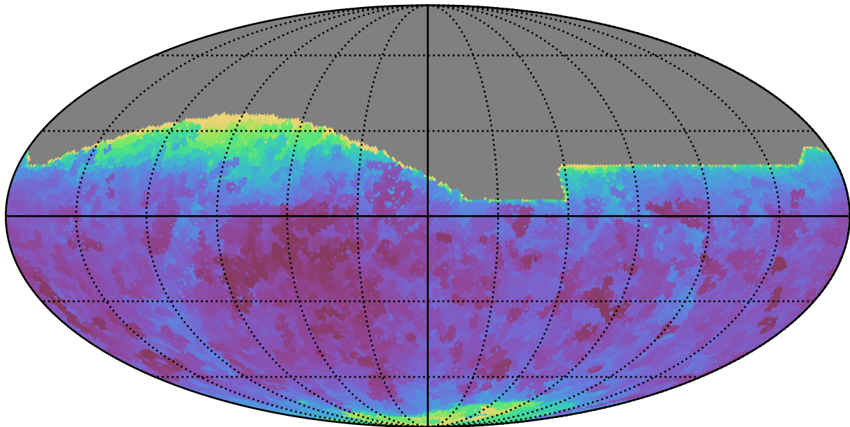
mw_roll_bulge_v3.3_10yrs All sky all bands: Min seeingEff
