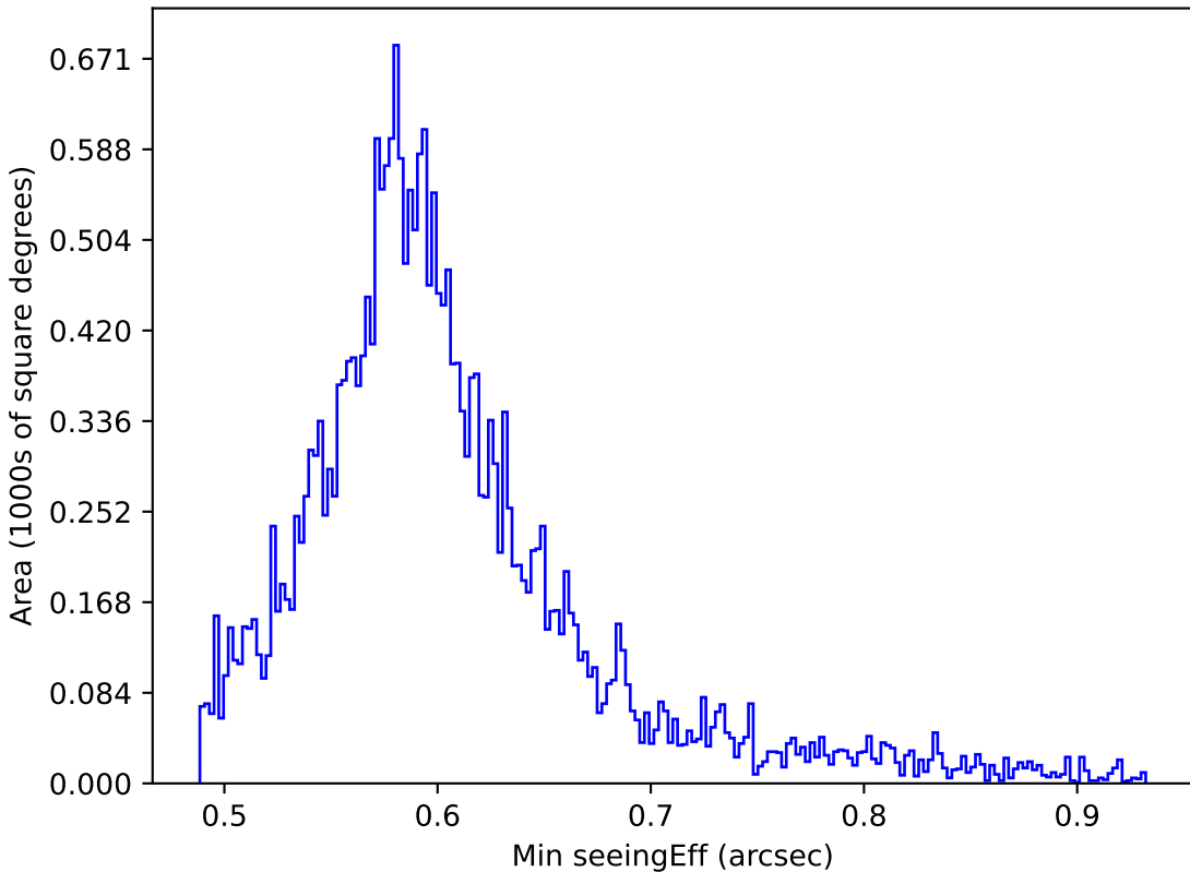
mw_roll_bulge_v3.3_10yrs All sky all bands: Min seeingEff
