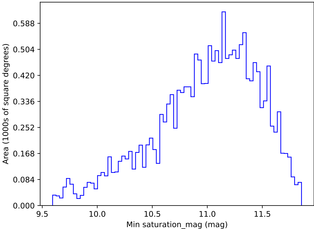
mw_roll_bulge_v3.3_10yrs WFD all bands: Min saturation_mag
