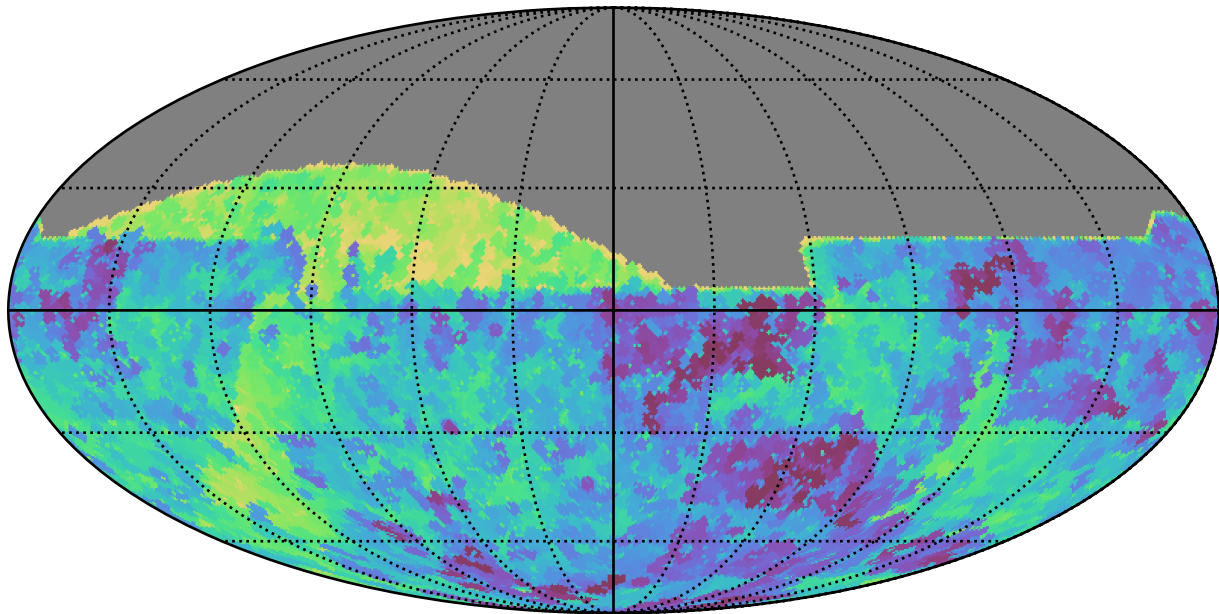
mw_roll_bulge_v3.3_10yrs All sky all bands: Min saturation_mag
