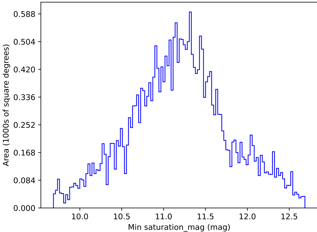
mw_roll_bulge_v3.3_10yrs All sky all bands: Min saturation_mag
