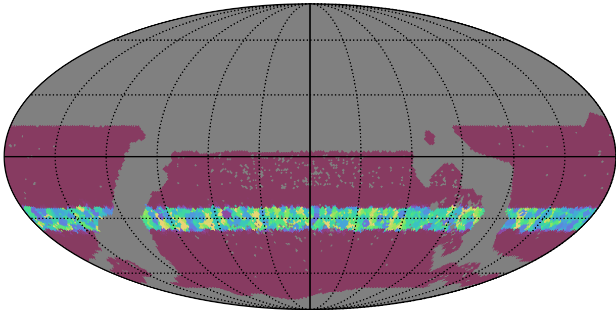
mw_roll_bulge_v3.3_10yrs WFD all bands: Min normairmass
