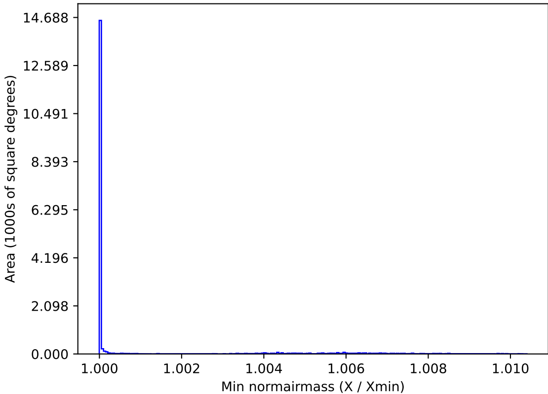
mw_roll_bulge_v3.3_10yrs WFD all bands: Min normairmass
