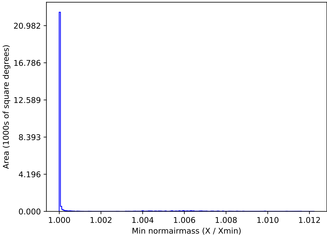
mw_roll_bulge_v3.3_10yrs All sky all bands: Min normairmass
