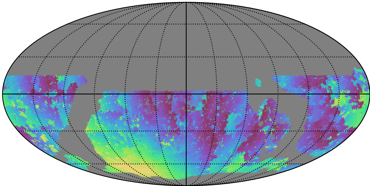
mw_roll_bulge_v3.3_10yrs WFD u band: Min moonDistance
