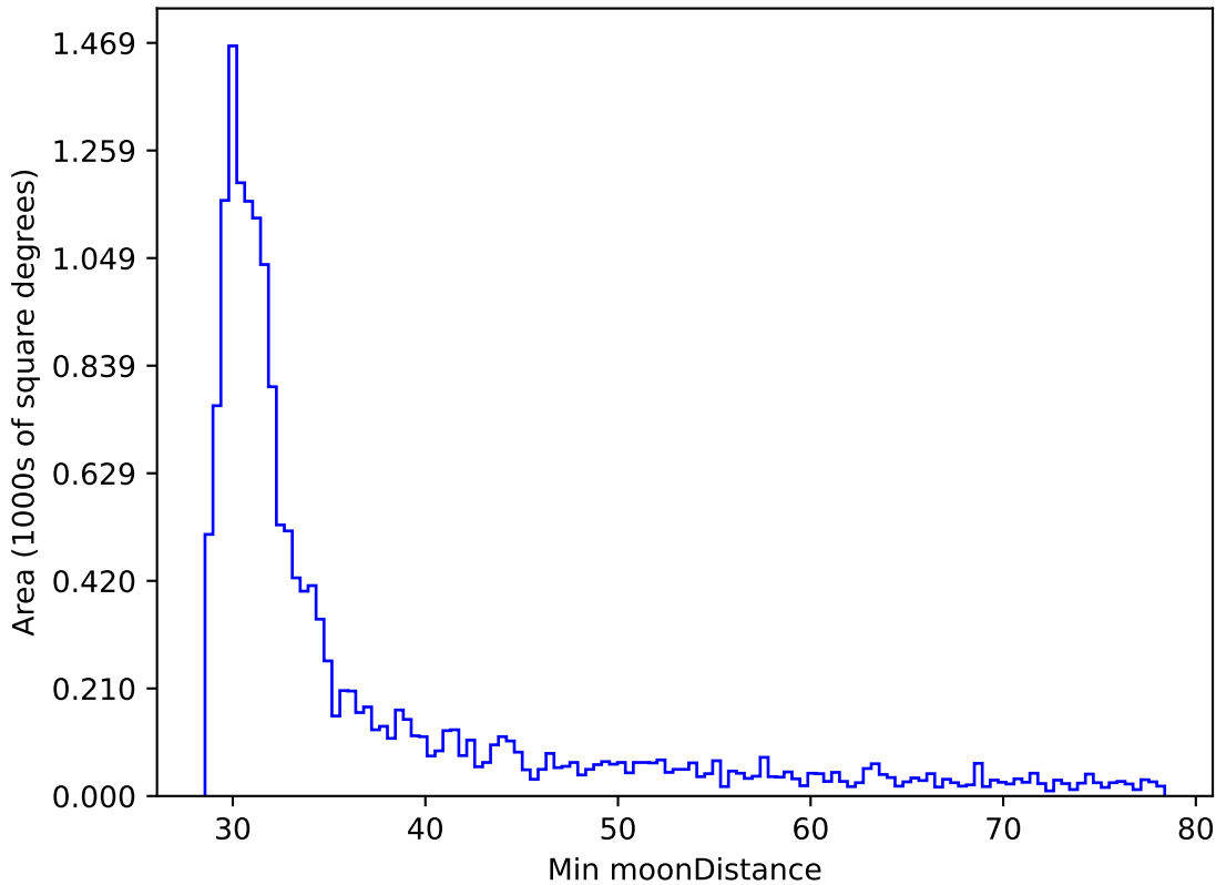
mw_roll_bulge_v3.3_10yrs WFD r band: Min moonDistance
