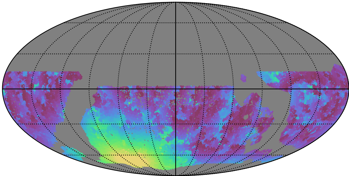
mw_roll_bulge_v3.3_10yrs WFD g band: Min moonDistance
