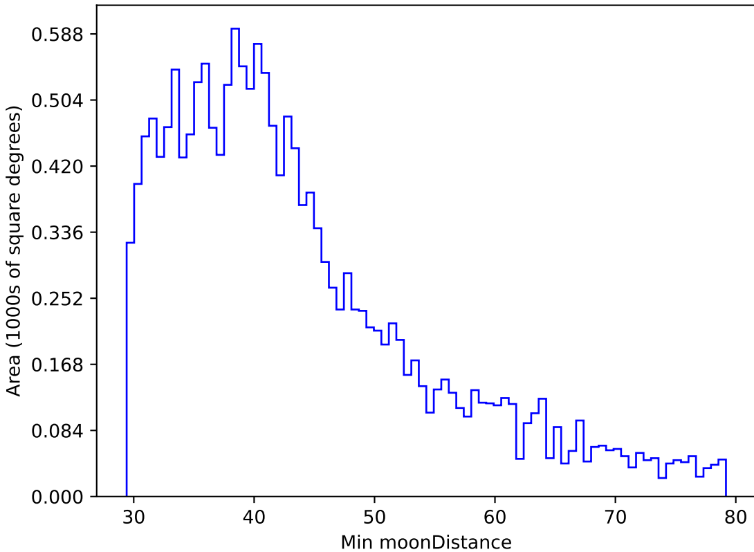
mw_roll_bulge_v3.3_10yrs WFD g band: Min moonDistance
