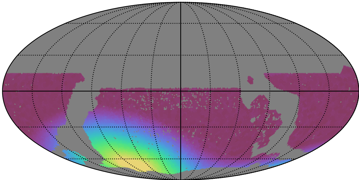
mw_roll_bulge_v3.3_10yrs WFD all bands: Min moonDistance
