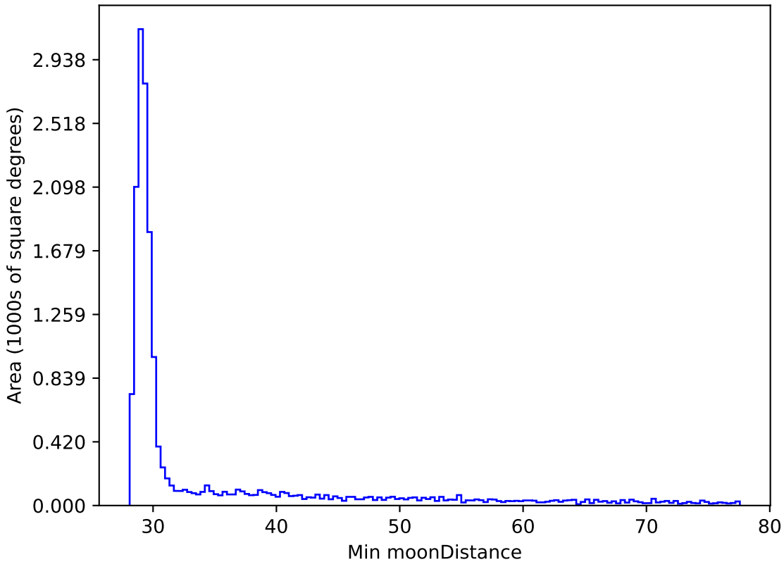
mw_roll_bulge_v3.3_10yrs WFD all bands: Min moonDistance
