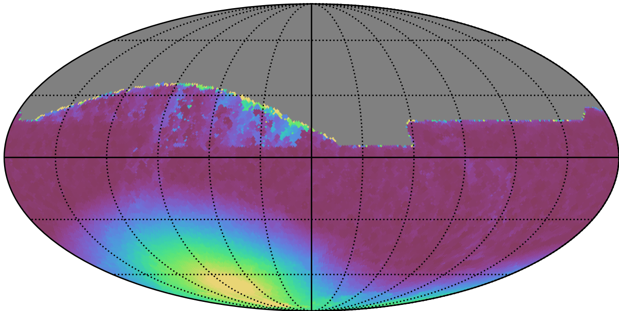
mw_roll_bulge_v3.3_10yrs All sky z band: Min moonDistance
