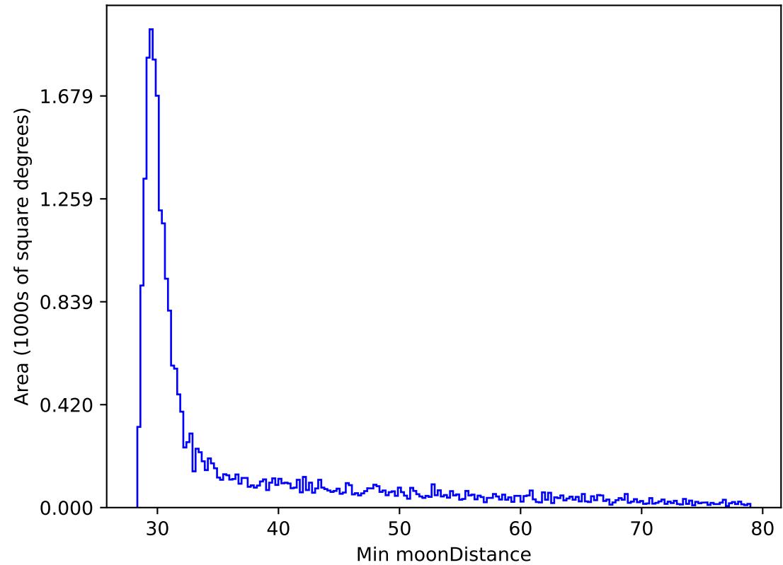
mw_roll_bulge_v3.3_10yrs All sky z band: Min moonDistance
