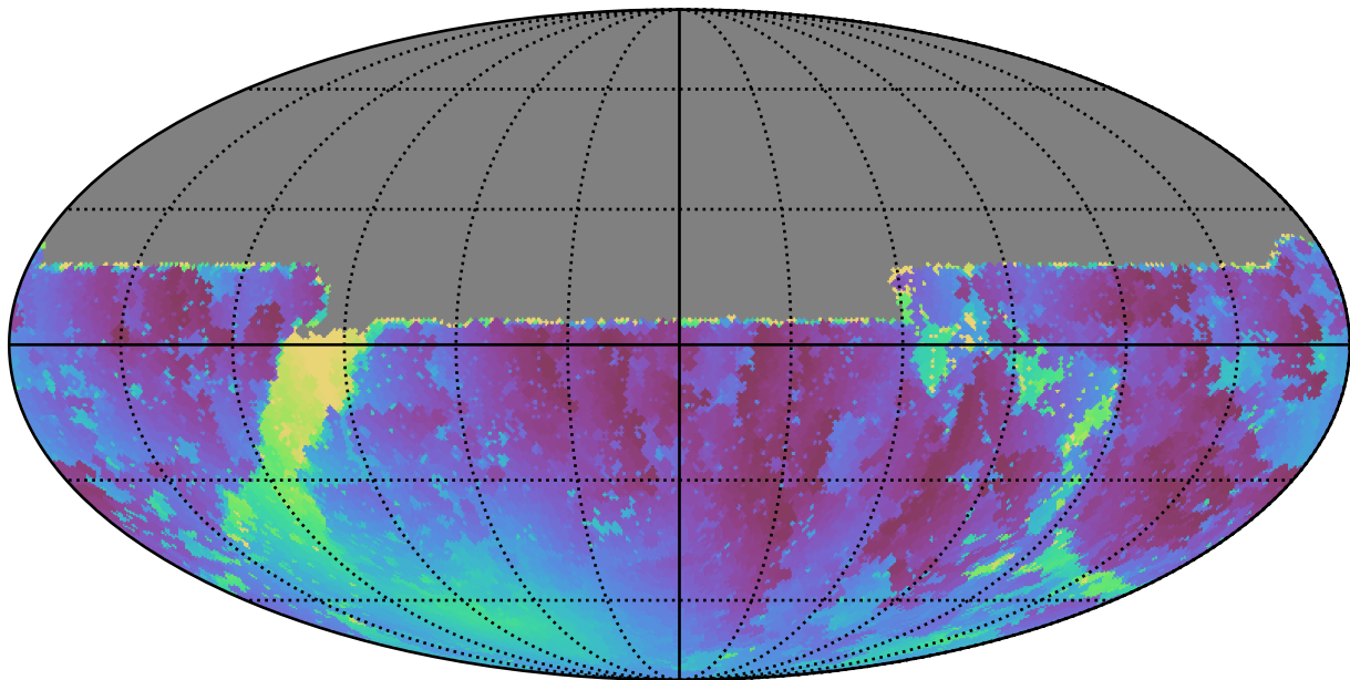
mw_roll_bulge_v3.3_10yrs All sky u band: Min moonDistance
