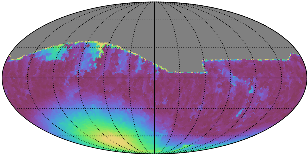
mw_roll_bulge_v3.3_10yrs All sky r band: Min moonDistance
