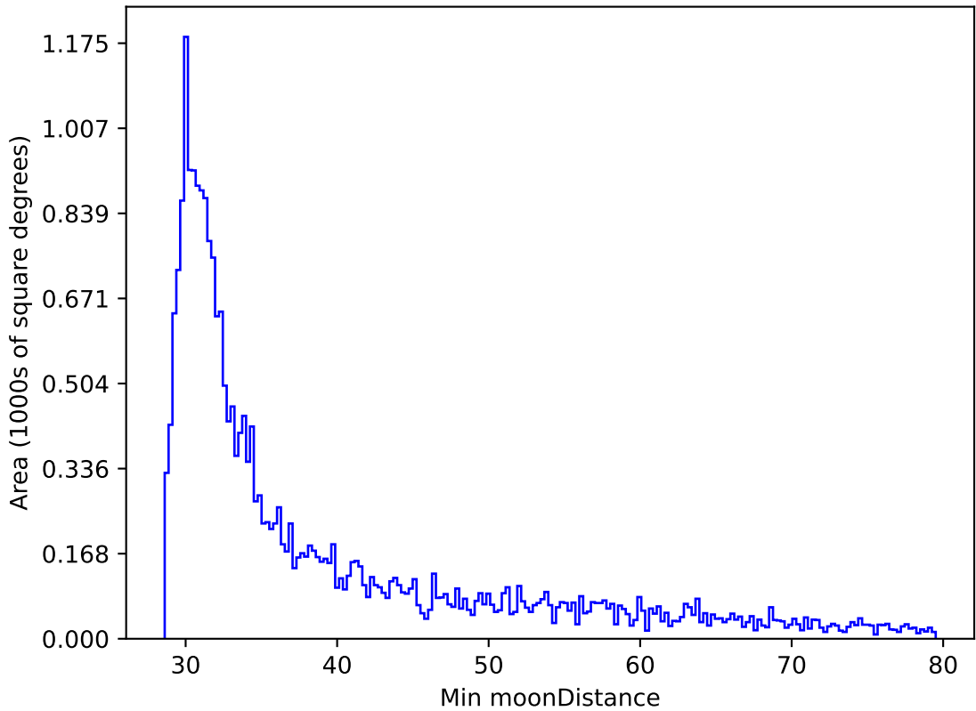
mw_roll_bulge_v3.3_10yrs All sky r band: Min moonDistance
