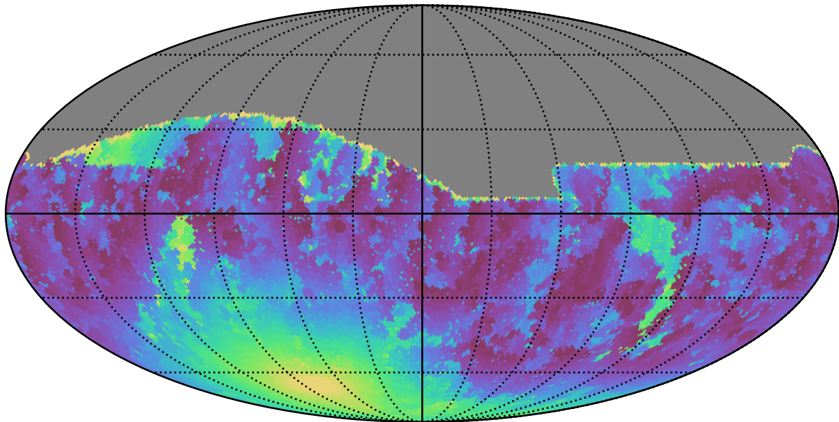
mw_roll_bulge_v3.3_10yrs All sky g band: Min moonDistance
