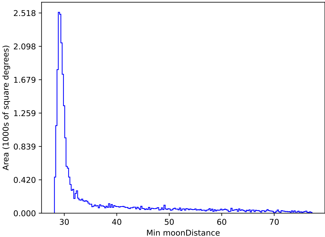
mw_roll_bulge_v3.3_10yrs All sky all bands: Min moonDistance
