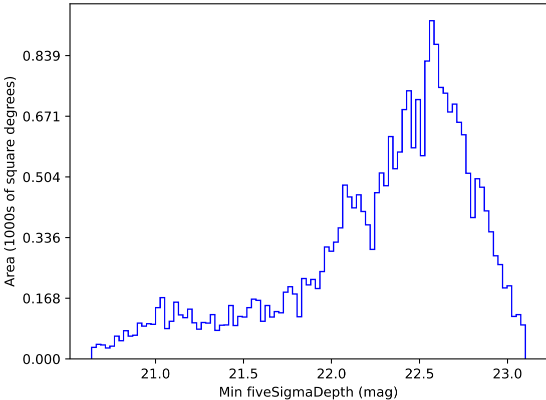
mw_roll_bulge_v3.3_10yrs Yr 1 z band: Min fiveSigmaDepth
