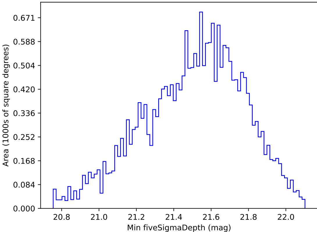
mw_roll_bulge_v3.3_10yrs Yr 1 y band: Min fiveSigmaDepth
