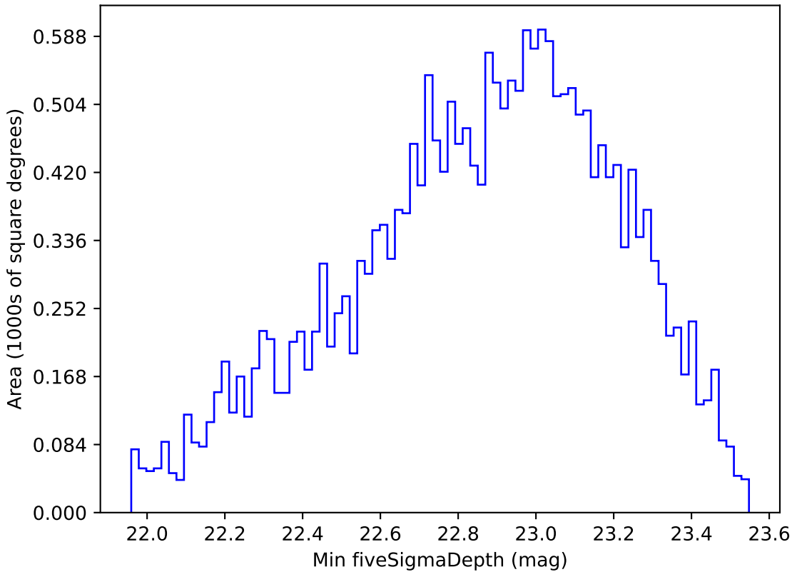
mw_roll_bulge_v3.3_10yrs Yr 1 u band: Min fiveSigmaDepth
