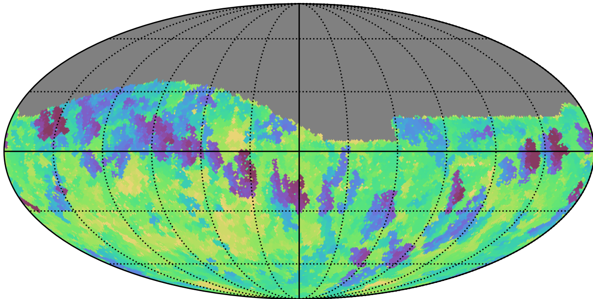
mw_roll_bulge_v3.3_10yrs Yr 1 i band: Min fiveSigmaDepth
