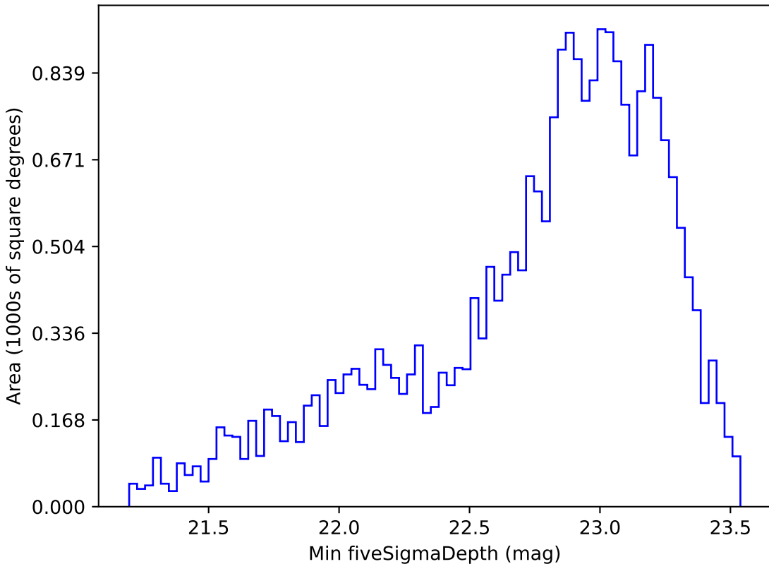
mw_roll_bulge_v3.3_10yrs Yr 1 i band: Min fiveSigmaDepth
