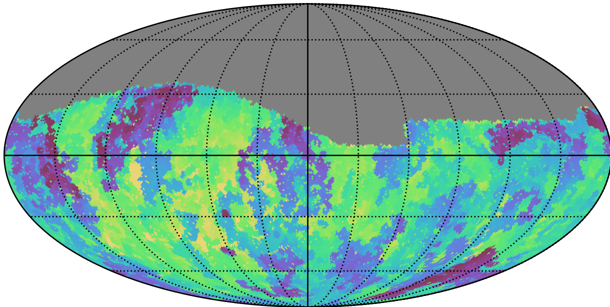
mw_roll_bulge_v3.3_10yrs Yr 1 g band: Min fiveSigmaDepth
