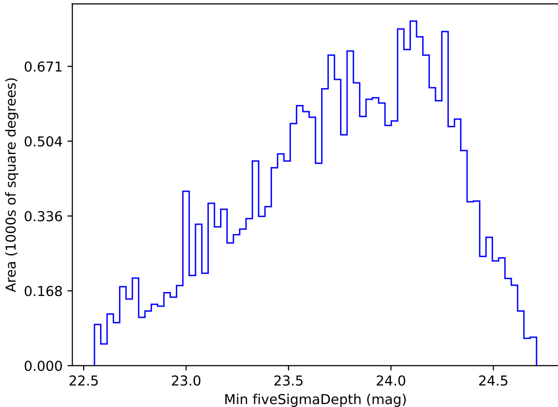
mw_roll_bulge_v3.3_10yrs Yr 1 g band: Min fiveSigmaDepth
