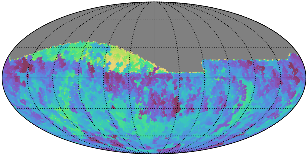
mw_roll_bulge_v3.3_10yrs Yr 1 all bands: Min fiveSigmaDepth
