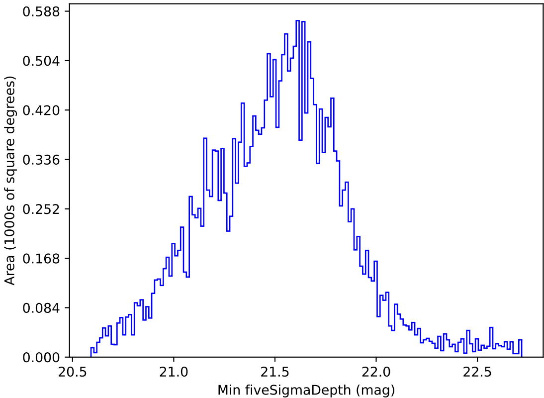
mw_roll_bulge_v3.3_10yrs Yr 1 all bands: Min fiveSigmaDepth
