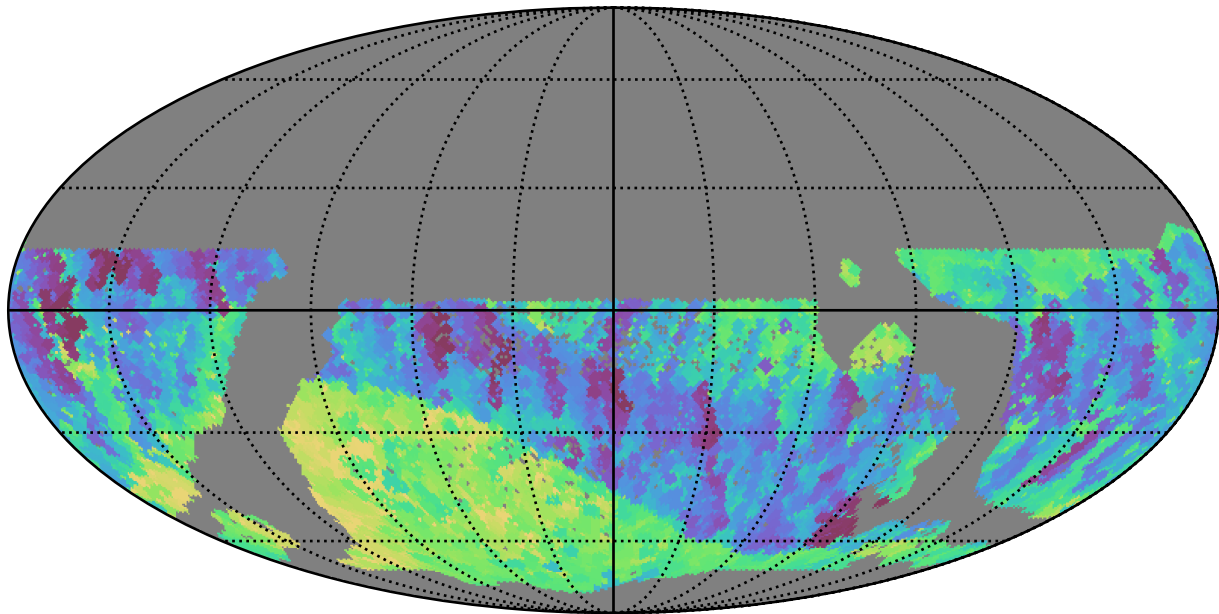
mw_roll_bulge_v3.3_10yrs WFD z band: Min fiveSigmaDepth
