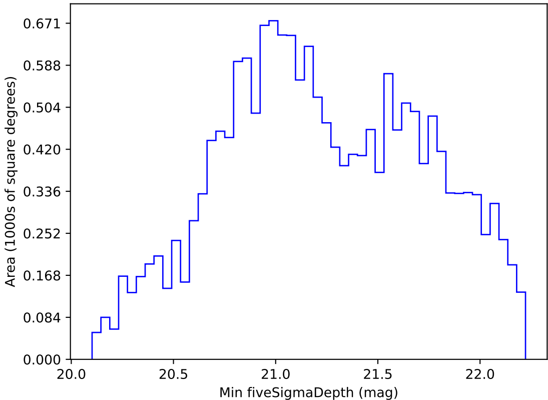
mw_roll_bulge_v3.3_10yrs WFD z band: Min fiveSigmaDepth
