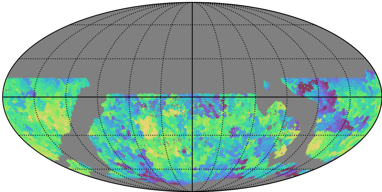
mw_roll_bulge_v3.3_10yrs WFD u band: Min fiveSigmaDepth
