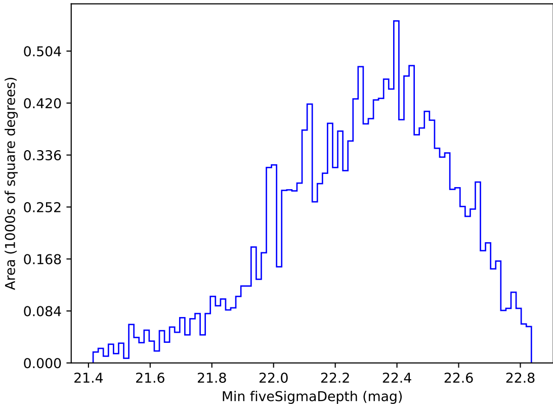
mw_roll_bulge_v3.3_10yrs WFD u band: Min fiveSigmaDepth
