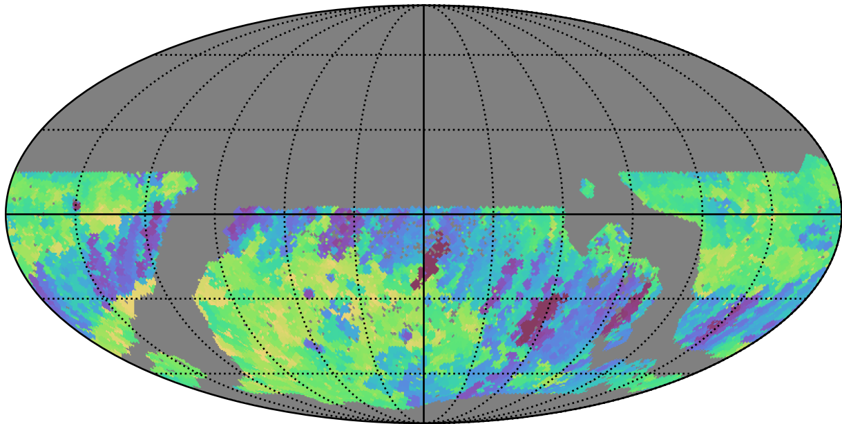
mw_roll_bulge_v3.3_10yrs WFD r band: Min fiveSigmaDepth
