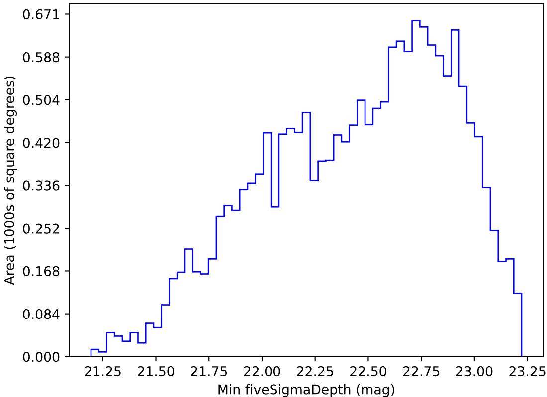
mw_roll_bulge_v3.3_10yrs WFD r band: Min fiveSigmaDepth
