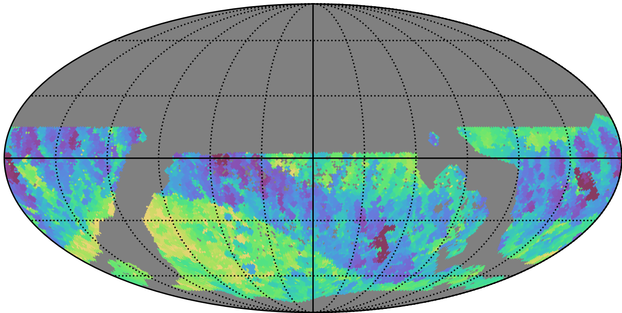
mw_roll_bulge_v3.3_10yrs WFD i band: Min fiveSigmaDepth
