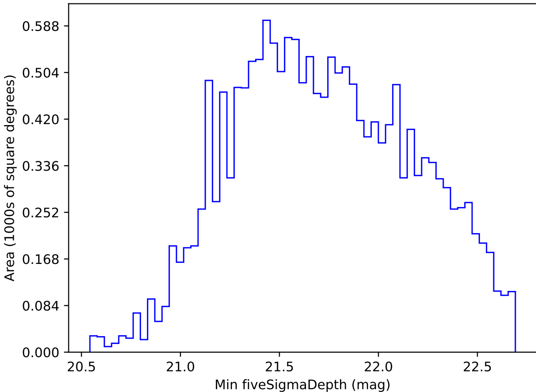
mw_roll_bulge_v3.3_10yrs WFD i band: Min fiveSigmaDepth
