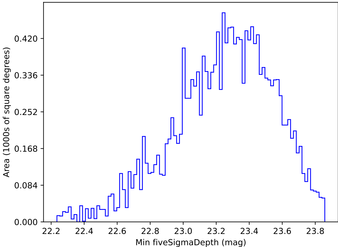
mw_roll_bulge_v3.3_10yrs WFD g band: Min fiveSigmaDepth
