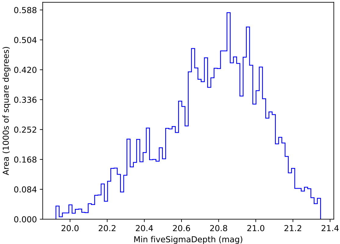
mw_roll_bulge_v3.3_10yrs WFD all bands: Min fiveSigmaDepth
