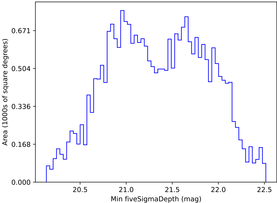
mw_roll_bulge_v3.3_10yrs All sky z band: Min fiveSigmaDepth
