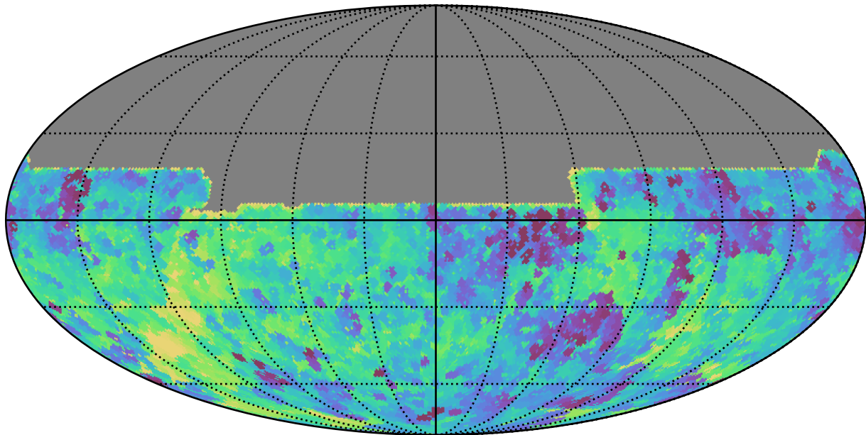
mw_roll_bulge_v3.3_10yrs All sky y band: Min fiveSigmaDepth
