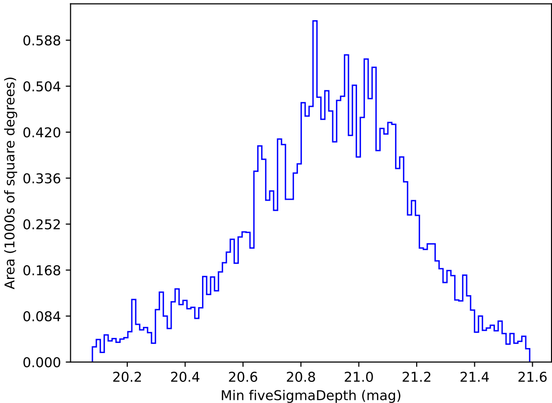
mw_roll_bulge_v3.3_10yrs All sky y band: Min fiveSigmaDepth
